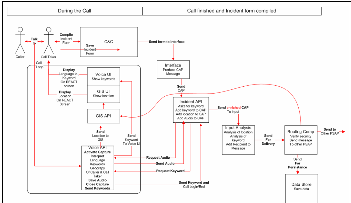
Figure 4. REACT Conceptual Sequence Diagram
